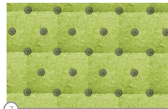
7 MINERAL WOOL – ANCHORS ARE PLACED CENTRALLY AND IN THE CORNERS OF THE NEIGHBOURING PANELS
